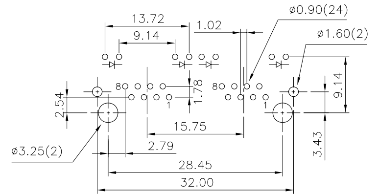
PCB LAYOUT (Ref.)
