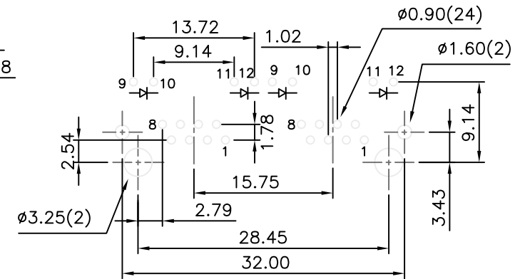
PCB LAYOUT (Ref.)
