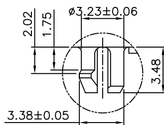
DETAIL X
