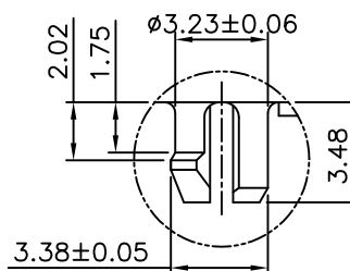
DETAIL X
