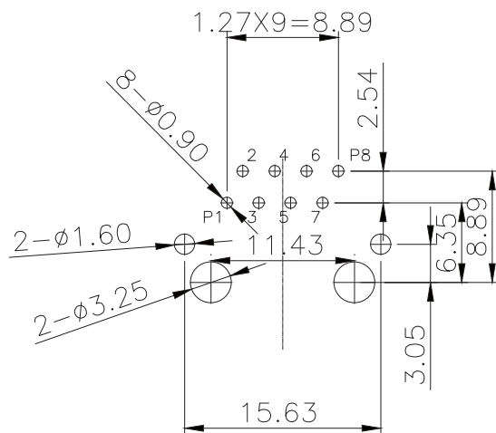
PCB LAYOUT
