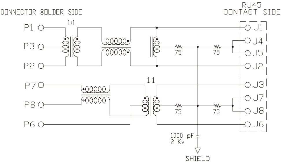
CONNECTOR SCHEMATIC
