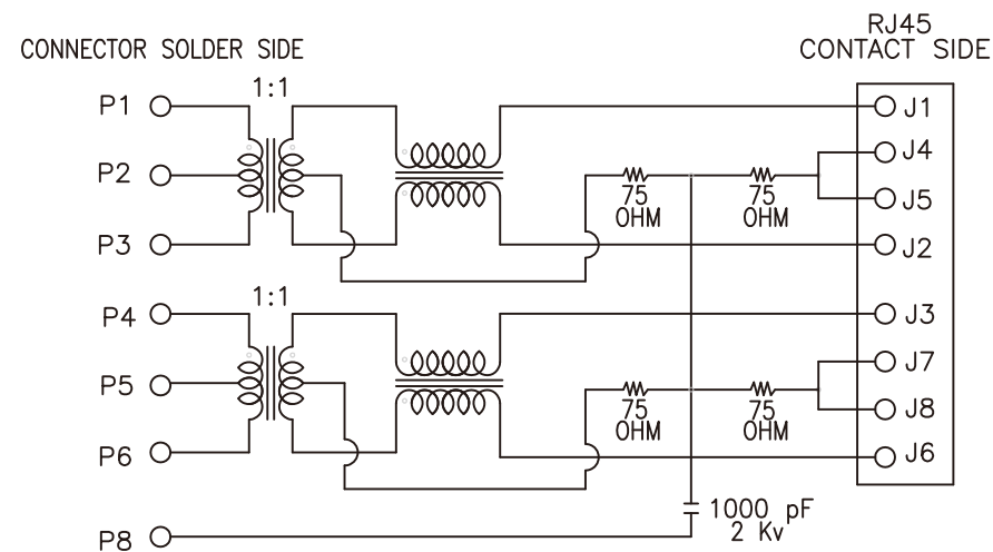
CONNECTOR SCHEMATIC
