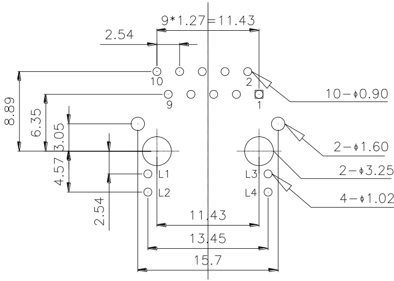
SUGGESTED PCB PAD LAYOUT COMPONENT SIDE VIEW
