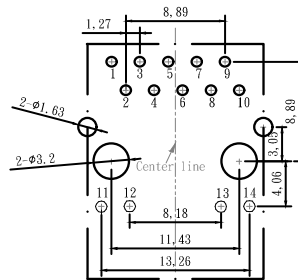
RECOMMENDED PCB LAYOUT VIEWED FROM COMPONENT SIDE
