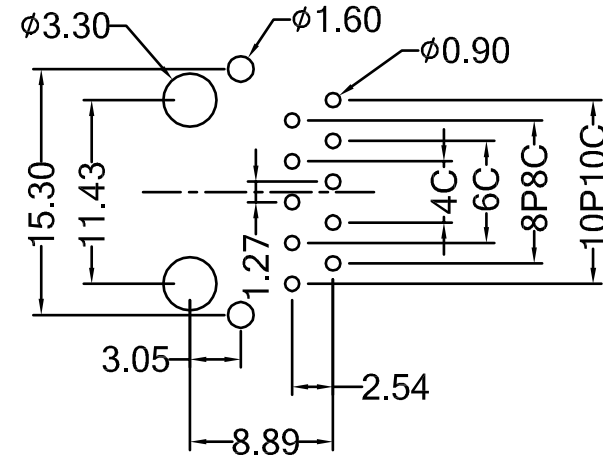
PCB LAYOUT / TOP VIEW / R3.05
