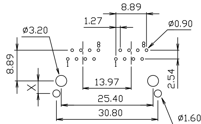
PC Board Layout Ref.
