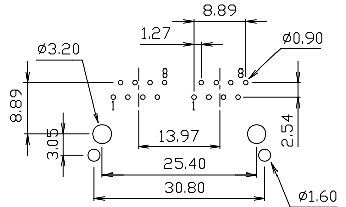
PC Board Layout Ref.
