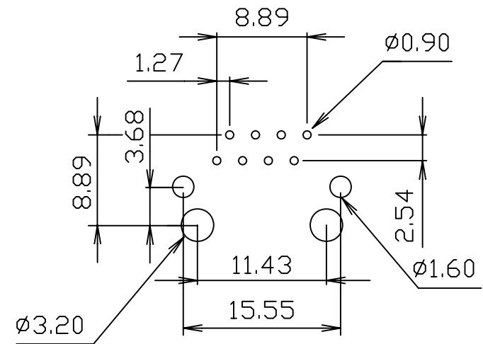
PC Board Layout
