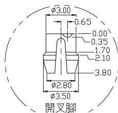
SPLIT-PEGS
