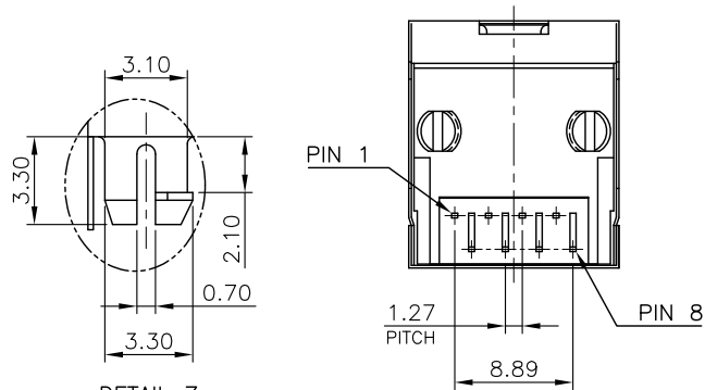
DETAIL Z SCALE 2:1
