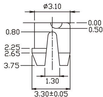
DETAIL X
