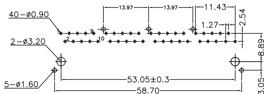
PCB LAYOUT/TOP VIEW
