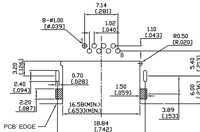
RECOMMENDED PCB LAYOUT TOP VIEW PCB THICKNESS: 1.60±0.05mm TOLERANCE: ±0.05mm
