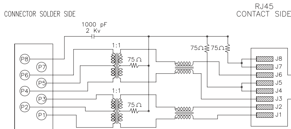
CONNECTOR SCHEMATIC
