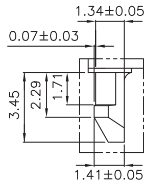
DETAIL X
