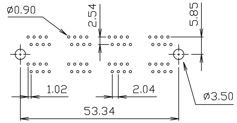
PCB LAYOUT
