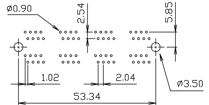
PCB LAYOUT
