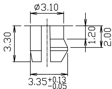
DETAIL X
