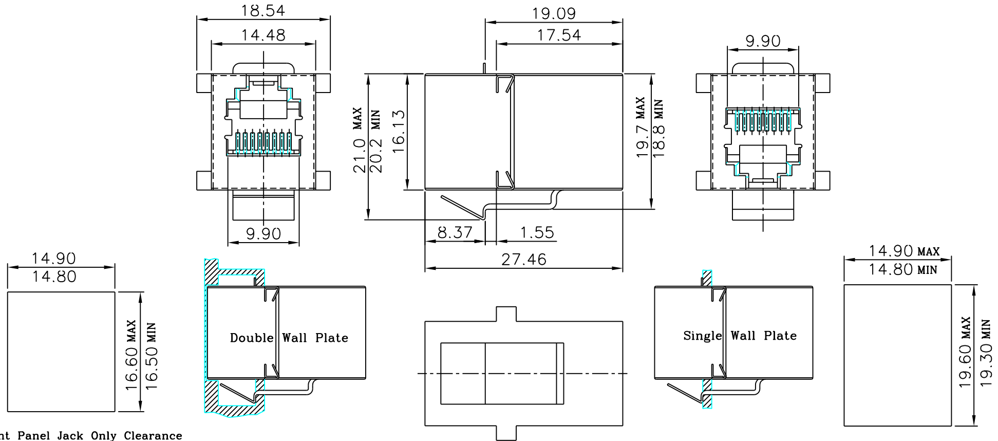
Single Panel-Latch Clearance Panel Thickness 0.062 inch
