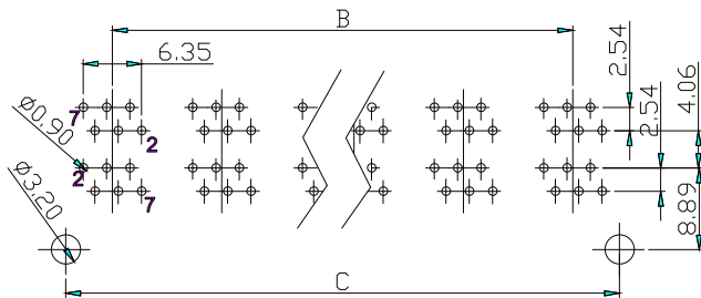
PC BOARD COMPONENT SIDE SHOWN
