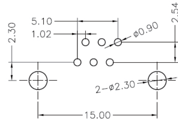
PCB Layout
