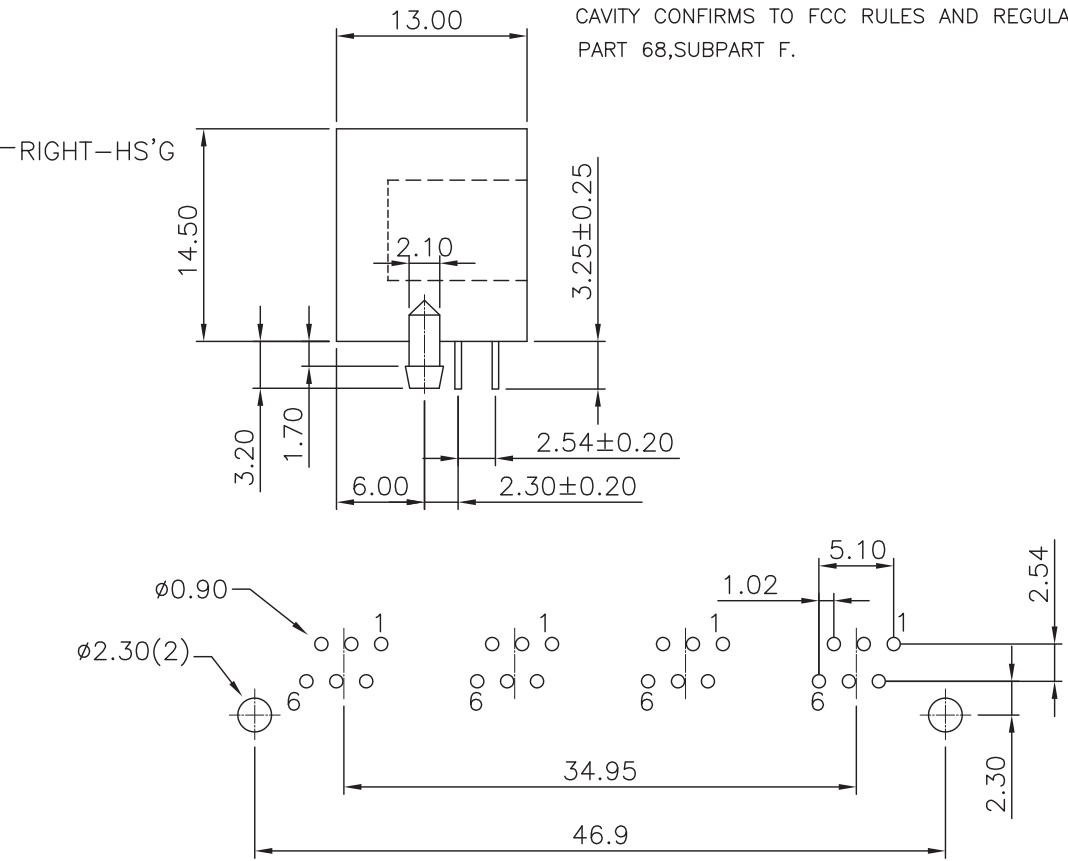
PCB LAYOUT Ref.
