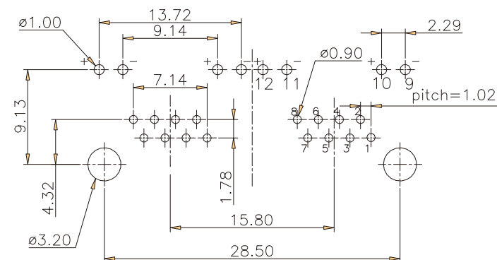
PCB Layout Component Side Shown
