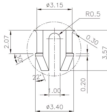
DETAIL "K"
