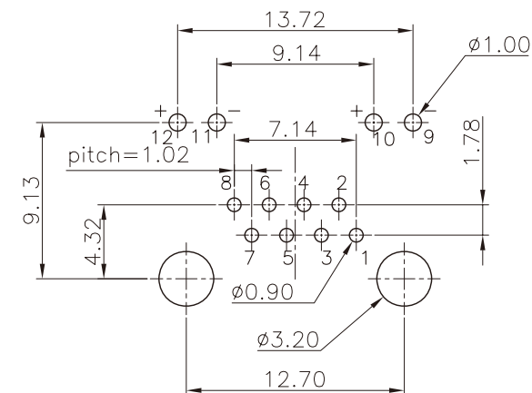
PCB LAYOUT COMPONENT SIDE SHOWN
