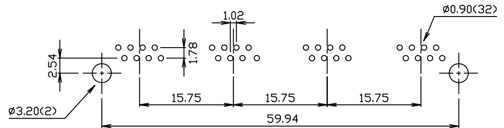
PCB LAYOUT
