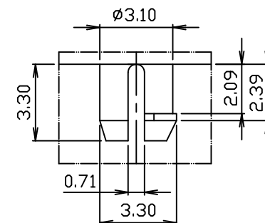
DETAIL X
