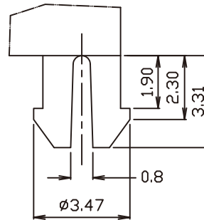
DETAIL X
