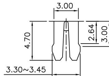
DETAIL X
