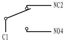
SCHMATIC DIAGRAM
