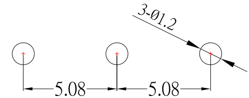
P.C.B LAYOUT MOUNTING
