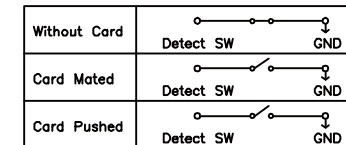
Circuit Diagram for Detect Switch
