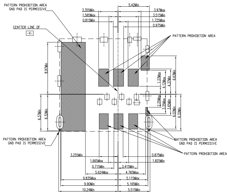
Recommended PCB Layout (General tolerance: \pm 0.05 )
