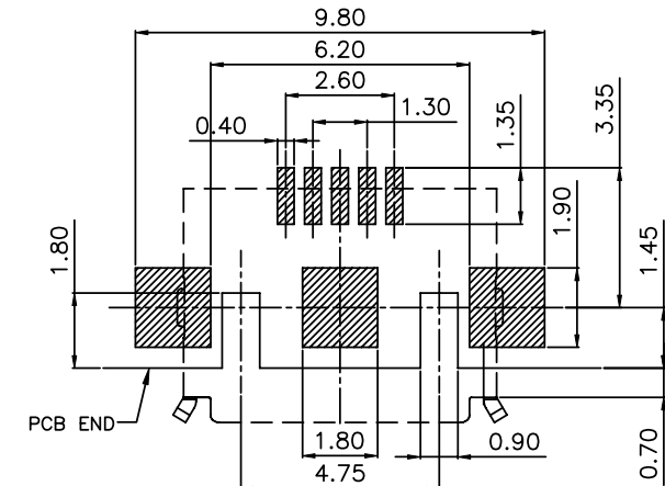
RECOMMENDED P.C. BOARD LAYOUT (TOLERANCE: ±0.05mm)
