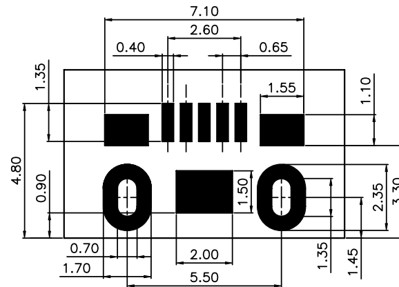
RECOMMENDED P.C.B. LAYOUT TOLERANCE \pm 0.03\text{mm}
