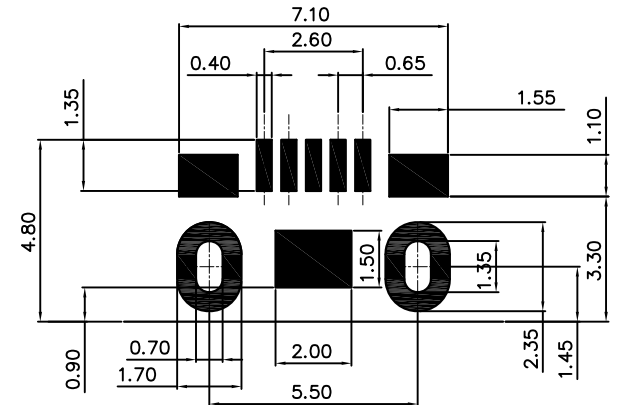
RECOMMENDED P.C.B. LAYOUT TOLERANCE ±0.03mm)
