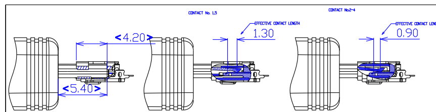
MATING VIEW
