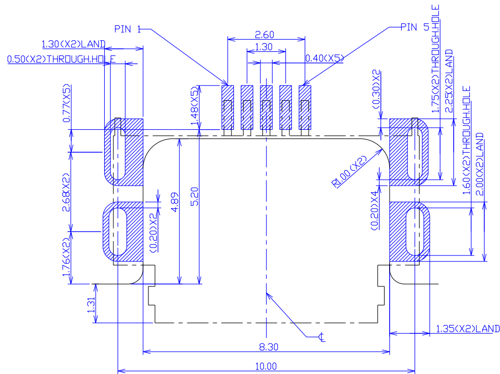
TOP VIEW RECOMMENDED PCB LAYOUT (TOLERANCE \pm 0.05\text{mm} )
