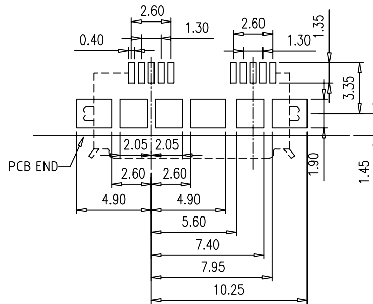
PCB Layout
