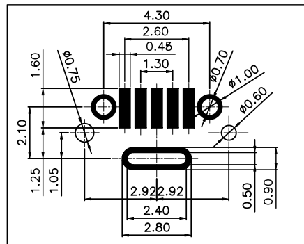
RECOMMENDED P.C.B. LAYOUT TOLERANCE \pm 0.03\text{mm}
