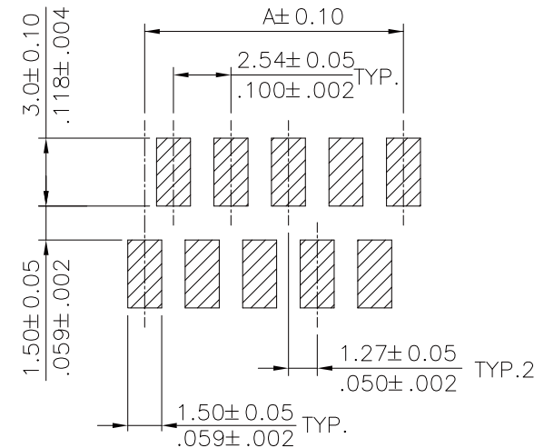
△ Solder Pad Pattern
