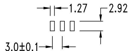
PCB Layout: Component side
