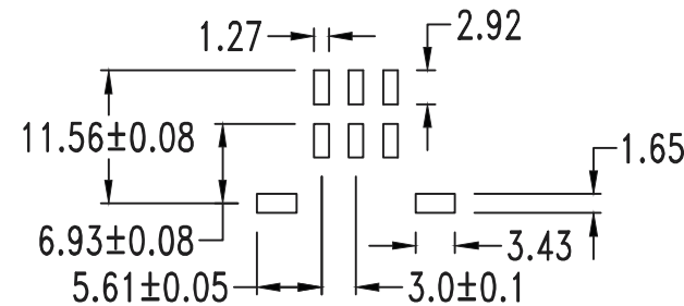
PCB Layout: Component side
