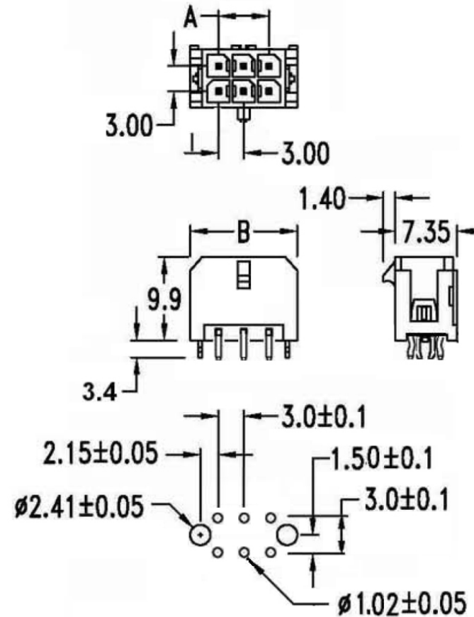
PCB Layout: Component side
