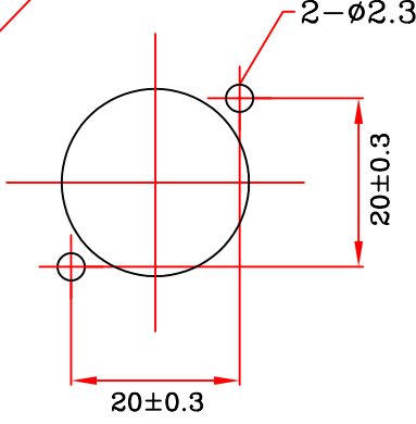
PANEL CUT OUT REAR VIEW
