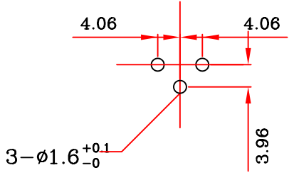
PCB-LAYOUT COMPONENT SIDE
