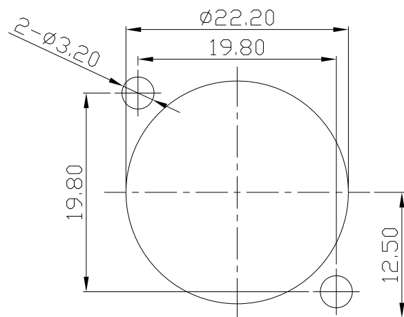
PANEL CUT OUT (FRONT SIDE)
