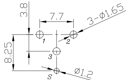
P.C.B. LAYOUT(±0.1) (TOP VIEW)
