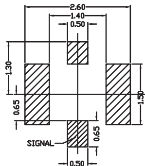
RECOMMENDED PCB LAYOUT (THK=1.6+/-0.15mm) (TOLERANCES ±0.05)
